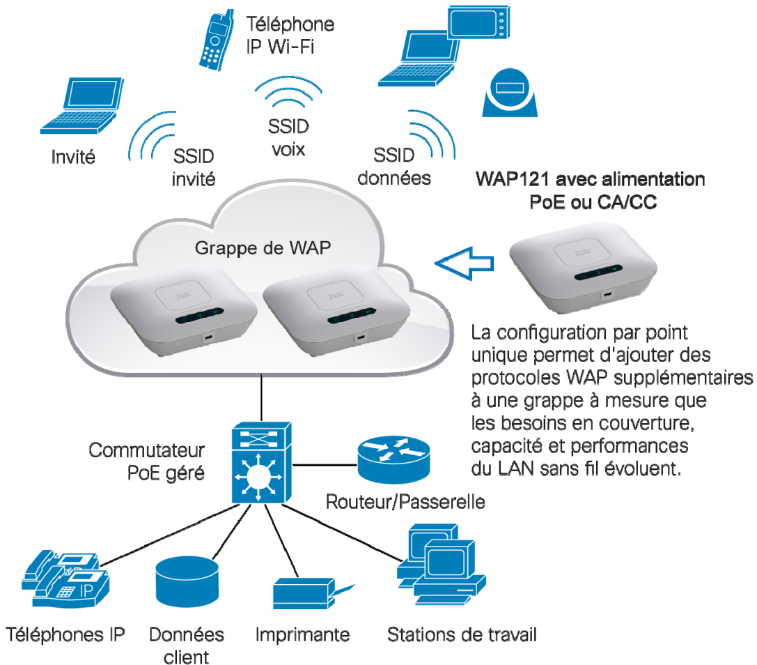
Figure 1. Configuration type
